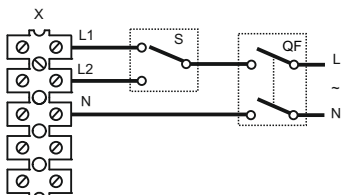
Wiring diagram 7
